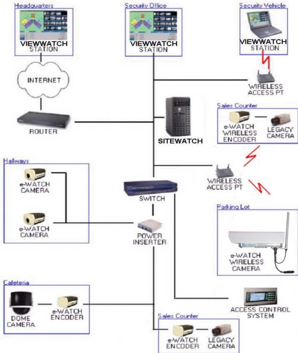
Figure 1-1 Typical e-Watch System
