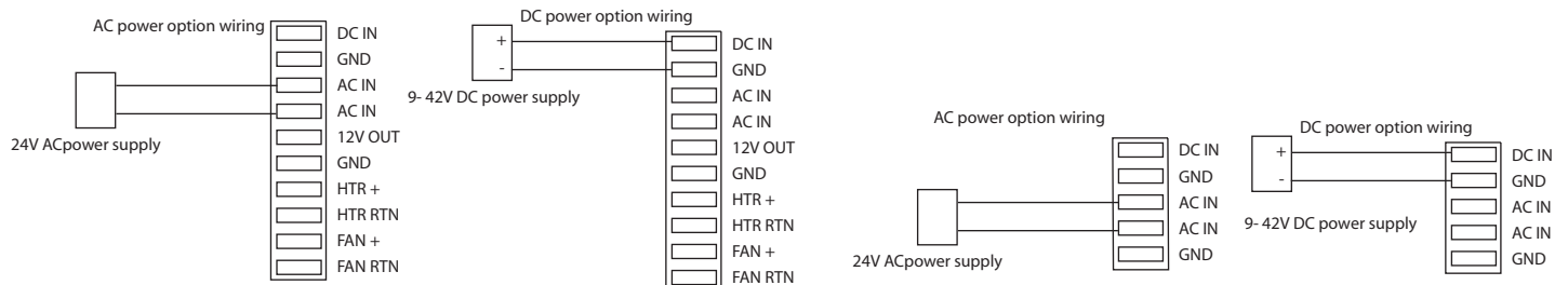
Five pin power plug wiring diagram.
